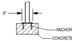
SURFACE FLANGE MOUNT (SF)
