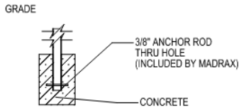
IN GROUND MOUNT (IG)
